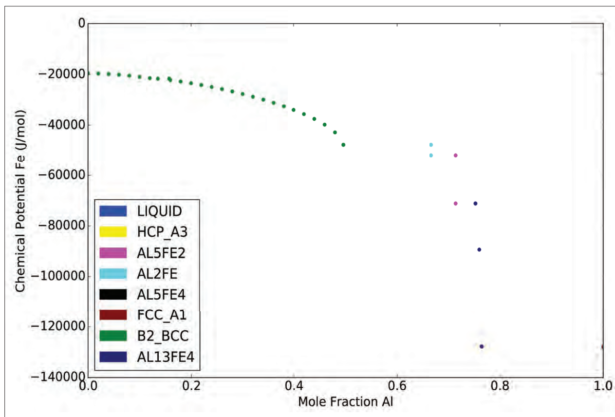
Figure 4: Equilibrium chemical potential of Fe as a function of Al composition in the Al-Fe system at 600 K, computed using pycalphad . Each point is color-coded with the corresponding stable phase; coexistence regions can be identified by the chemical potential remaining at across a range of composition. The end-points of such an iso-potential region can be directly connected to the corresponding tie-line at the given temperature.
