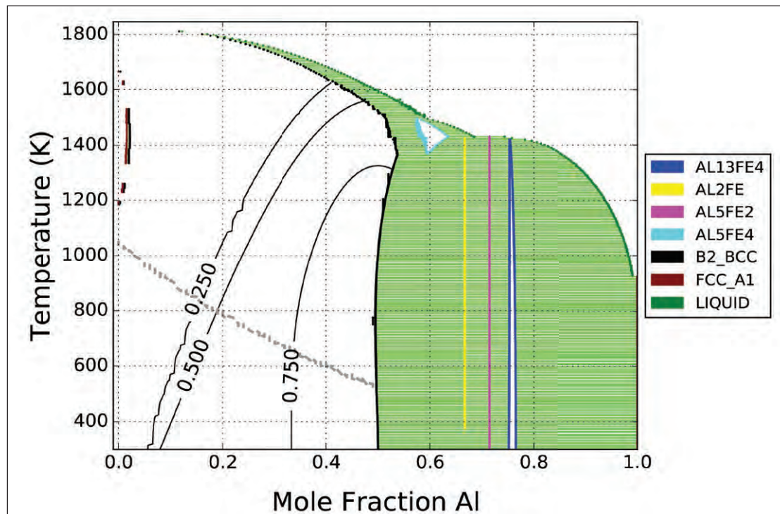
Figure 5: Phase diagram of the Al-Fe system according to the COST 507 database, computed using pycalphad. The solid black lines in the B2 region correspond to lines of constant “degree of ordering” in the B2 phase. The grey dashed line is the Curie temperature. The bcc ordering transition is second-order since the degree of ordering is continuously changing with respect to composition and temperature. Some lines in the diagram are not smooth due to the coarseness of the grid used in the calculation; mapping in pycalphad is still experimental.
