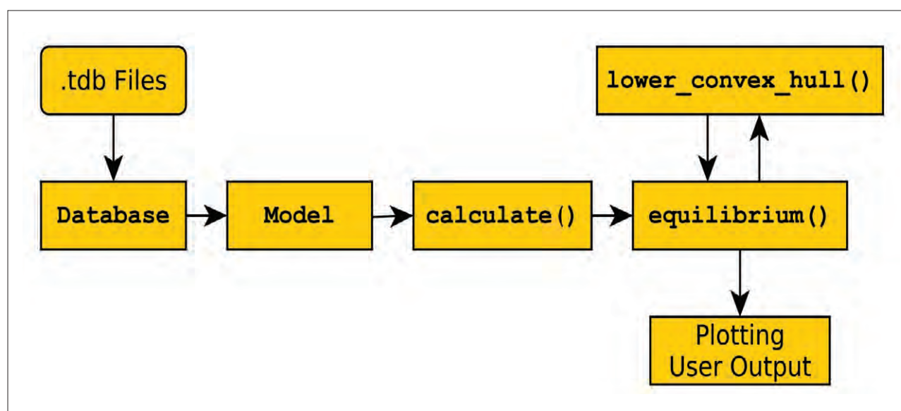
Figure 1: General architecture of the pycalphad software package. Using parameters from the given Database , a Model object is constructed for each phase and then fed into the calculation engine to produce results for the user.
